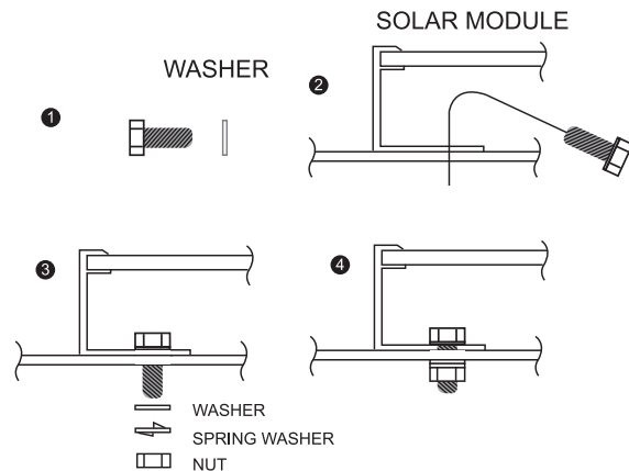
Figure 2 Mounting Details
